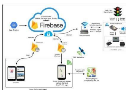
Gambar 4. Desain Sistem Smart Traffic Light
